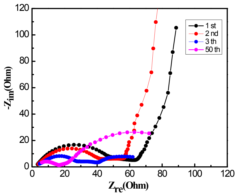
Fig. S2 Nyquist plots of \text{Li}_4\text{Ti}_5\text{O}_{12} anodes in \text{LiTFSi/ethers} electrolyte after different cycles at the rate of 2C.
