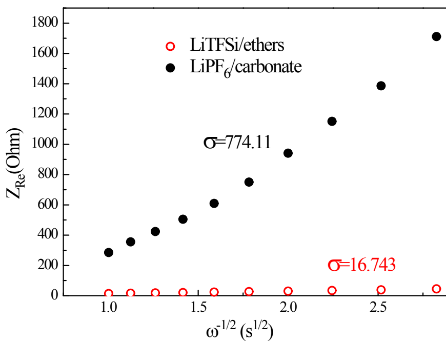
Fig. S1 Z_{Re} vs \omega^{-1/2} plots in the low frequency region obtained from EIS measurements.
