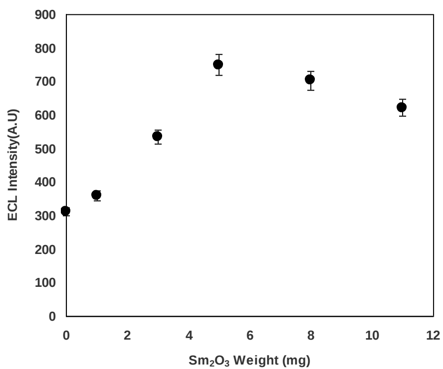
Fig.S4. Effect of \text{Sm}_2\text{O}_3 on the ECL intensity
