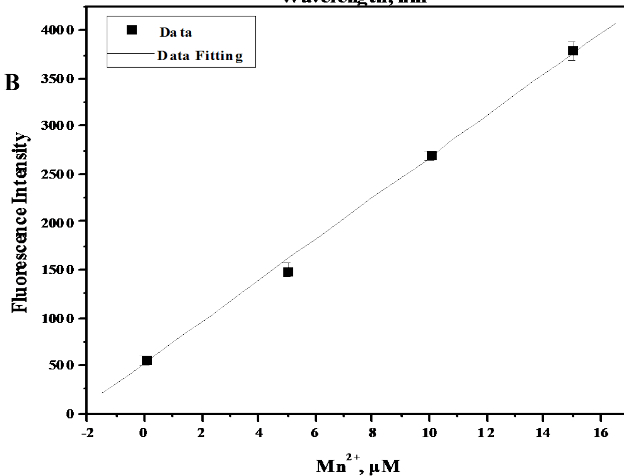
Figure S1. (A) Fluorescence responds upon addition different [Mn] and (B) linear relationship of the fluorescence changes and [Mn]
