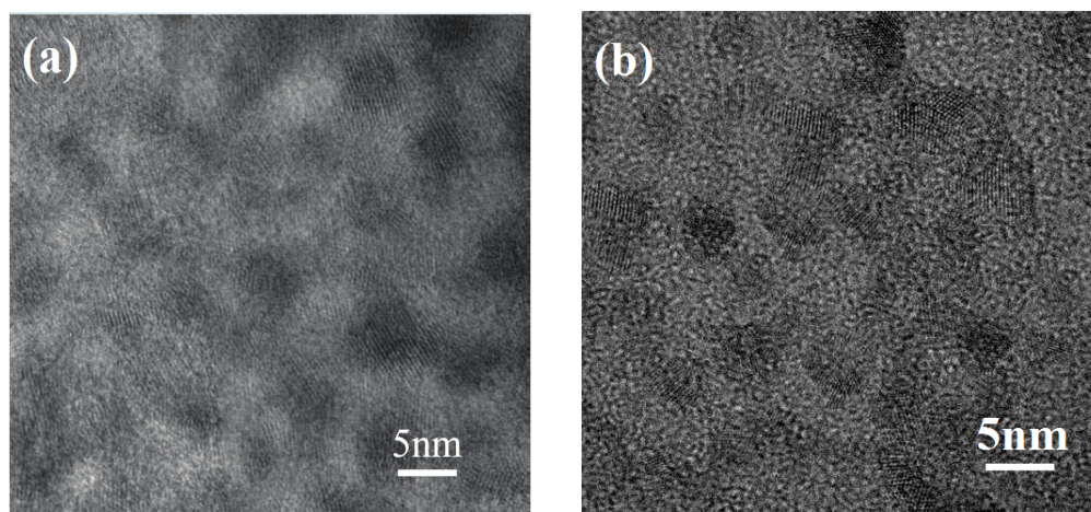
Fig.S1 (a) TEM of the TGA/ZnS QD , (b)TEM of the L-Cys/ZnS QDs.
