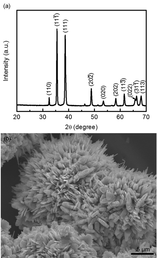
Fig. S1 XRD pattern and SEM image of CuO nanoplatelets.
