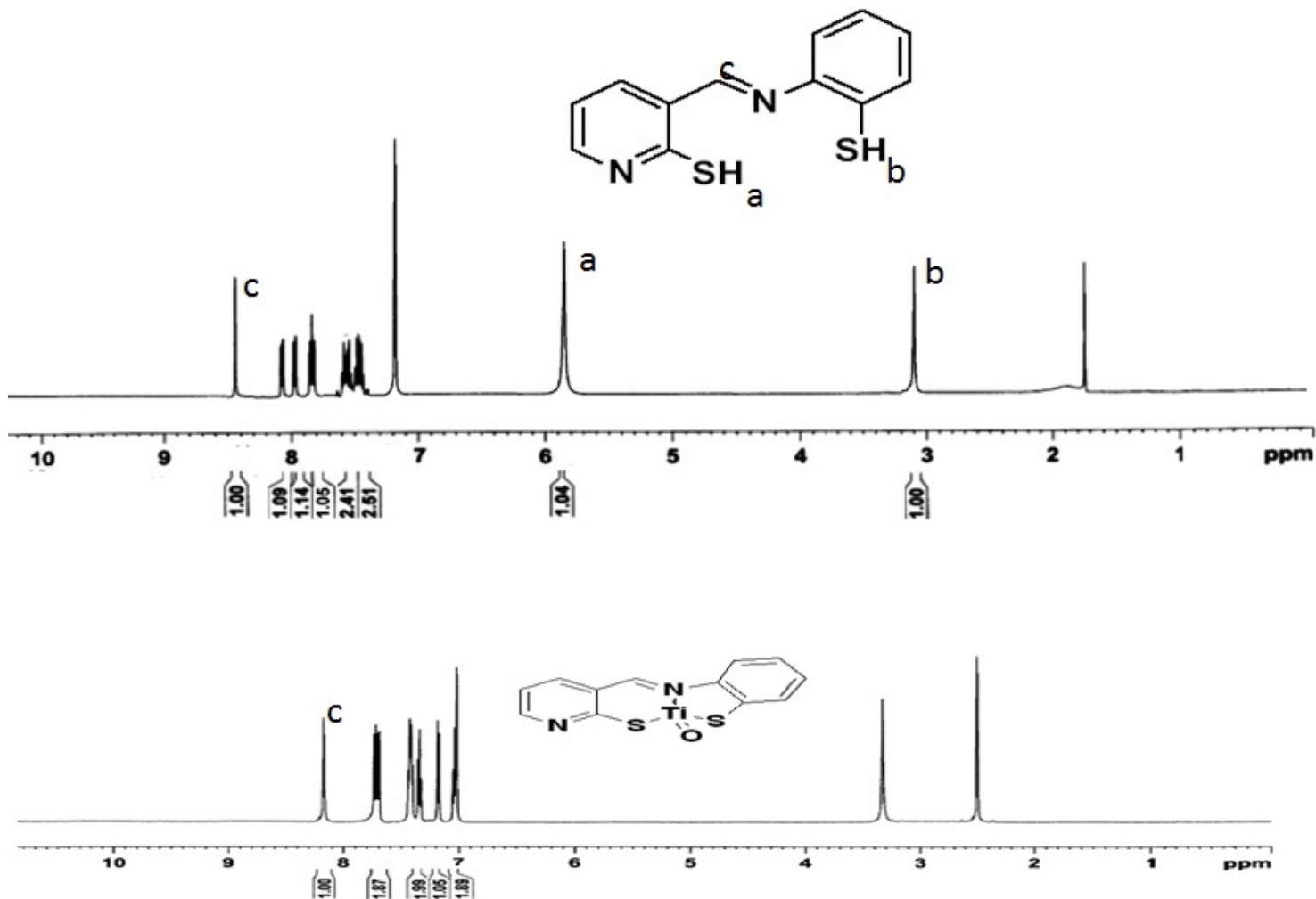
Figure S7: ^1\text{H-NMR} spectra of MPPT and Ti(MPPT)O
