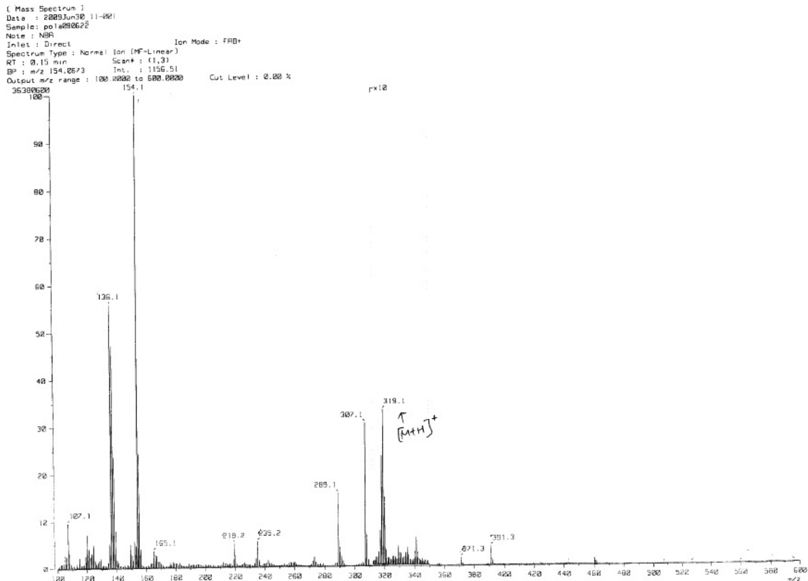
Figure S9: Mass spectrum of Methylene blue sample after 20 minutes of Visible light irradiation
