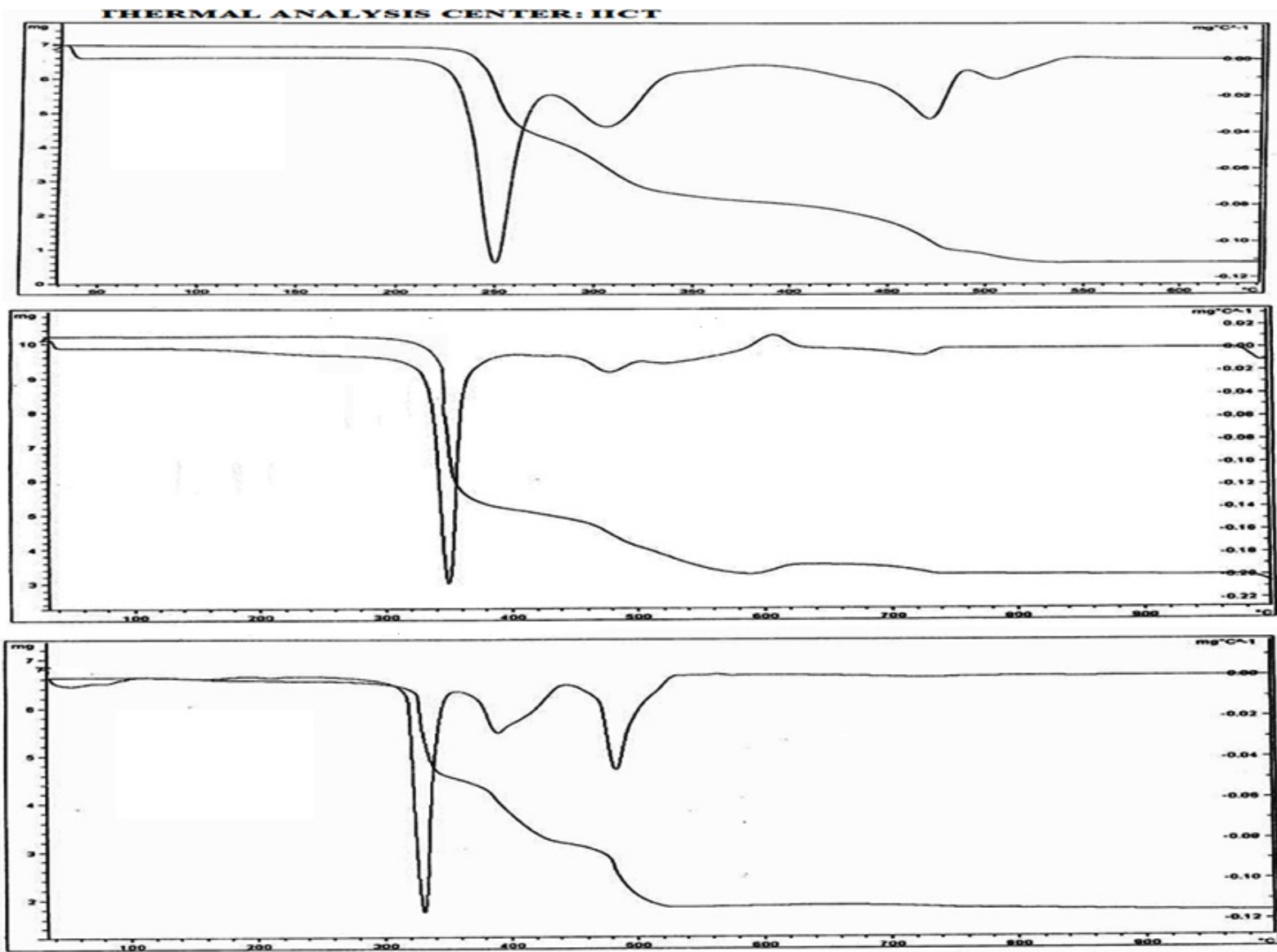
Fig. S2 Thermograms of Ti(MPPT)O, Ti(DMPMPT)O and Ti(DCMPPT)O
