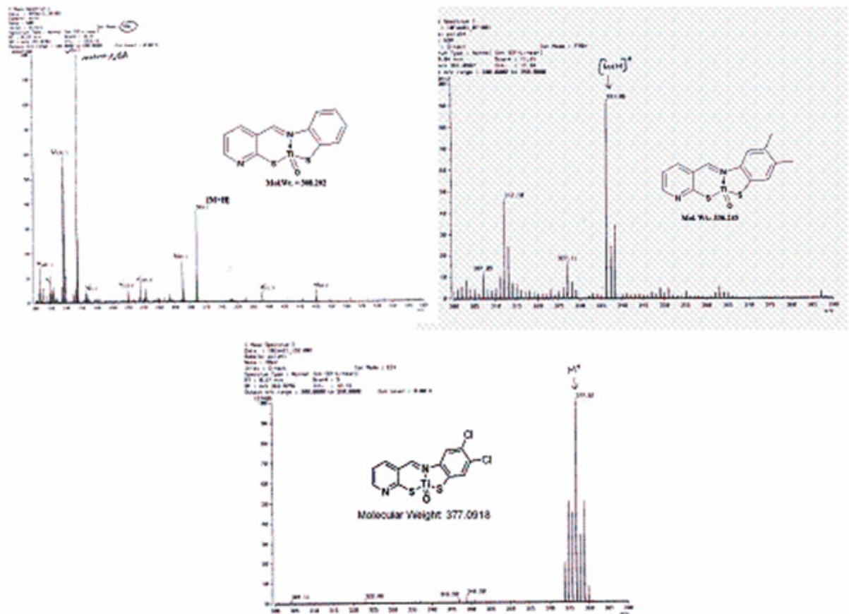
Figure S3: Mass spectra of Ti(MPPT)O, Ti(DMPMPT)O and Ti(DCMPPT)O
