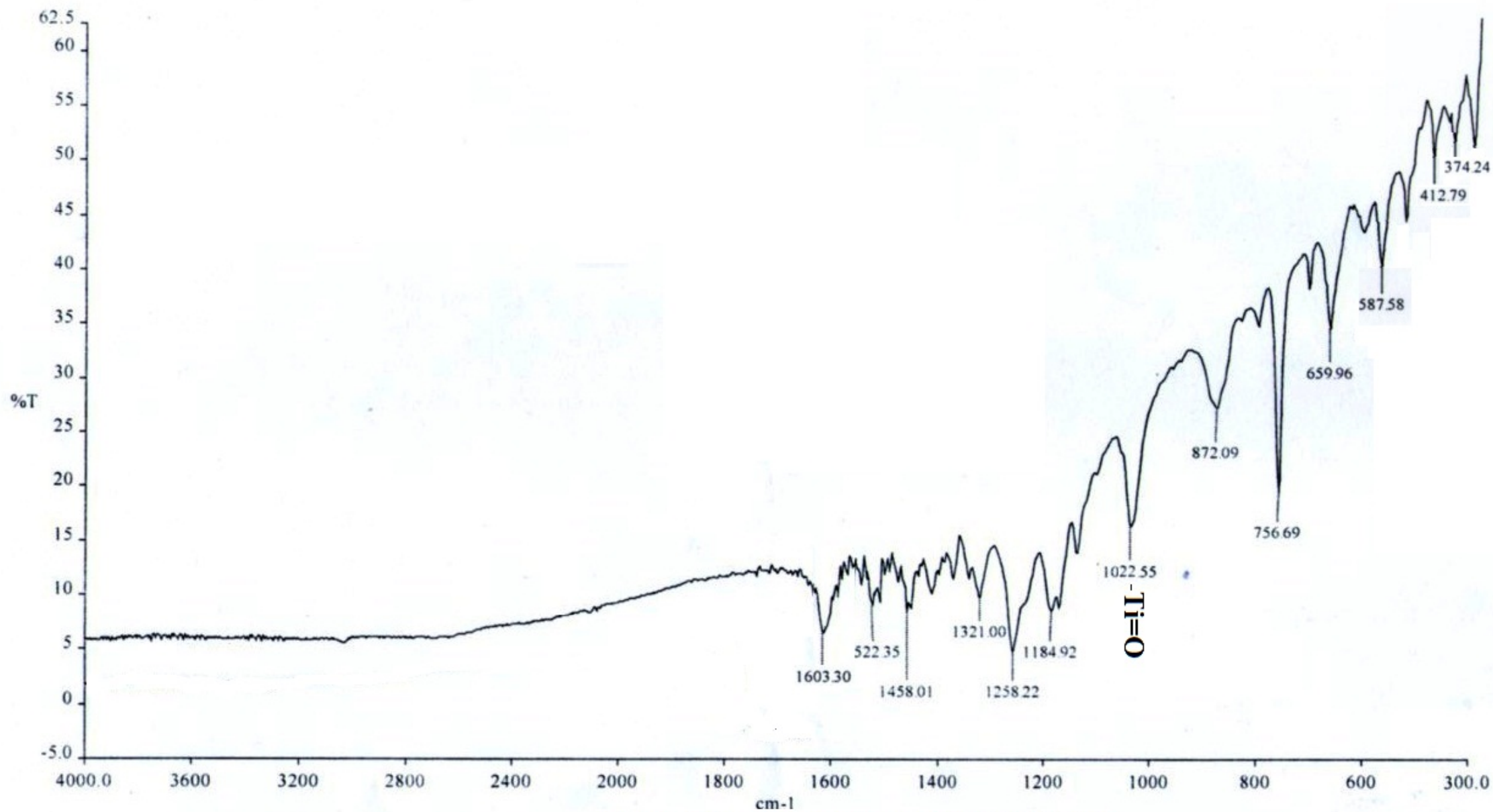
Figure S4-a: IR spectrum of Ti(MPPT)O
