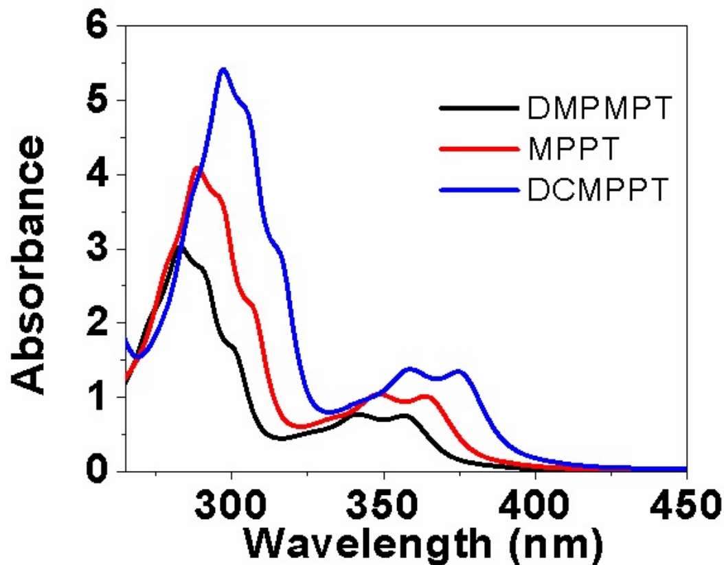
Figure S5: UV spectra of MPPT, DMPMPT and DCMPT
