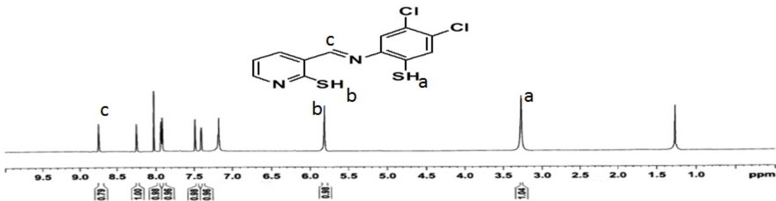
Figure S6: 1 H-NMR spectra of DMPMPT and DCMPT
