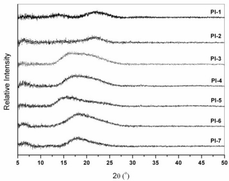
Fig. 2 Wide-angle X-ray diffractograms of the polyimide films.
