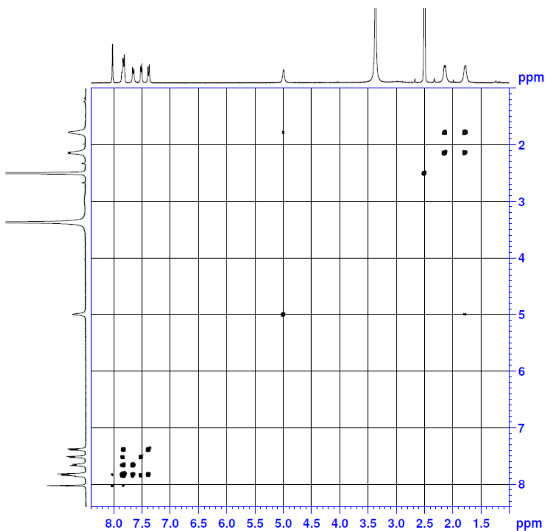
Figure S1. COSY spectrum of PI-2 in DMSO- d 6
