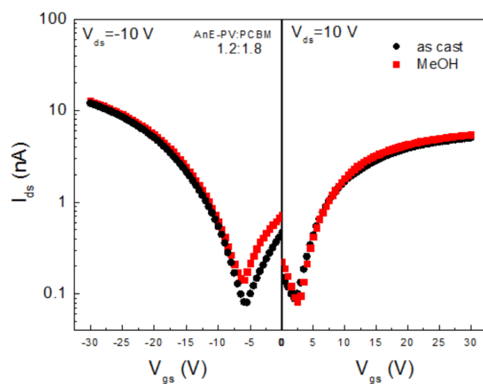
Fig S1. Transfer characteristics of OFETs with AnE-PV :PCBM (1.2 :1.8) as active layer with and without methanol treatment.
