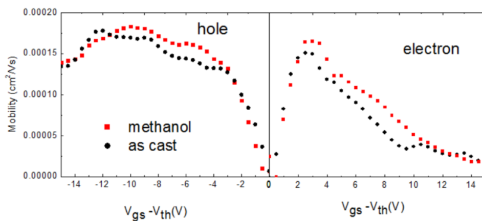
Fig S2. Derived gate voltage dependant mobilities in saturation regime.
