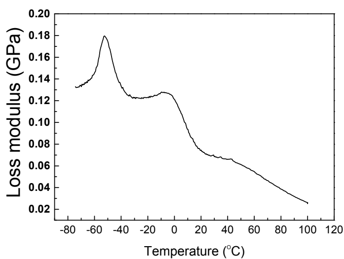
SFig.2 DMA loss modulus-temperature curves of the IPC.
