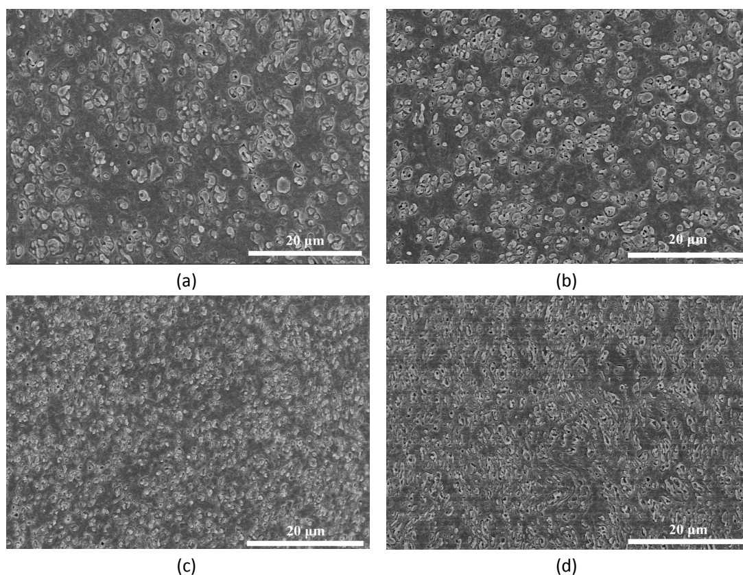
SFig.1 SEM micrographs of YZ plane of A2 (a), A3 (b), B2 (c) and B3 (d), Z is horizontal.
