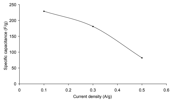
Figure S3. Specific capacitance of \text{Mn}_3\text{O}_4 hexagonal plates (sample S6) at different current densities.
