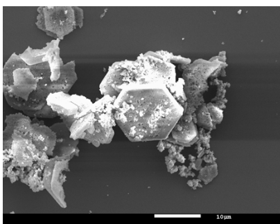
Figure S2. FE-SEM image of \text{Mn}_3\text{O}_4 hexagonal plates (sample S6) after 4 minutes sonication.
