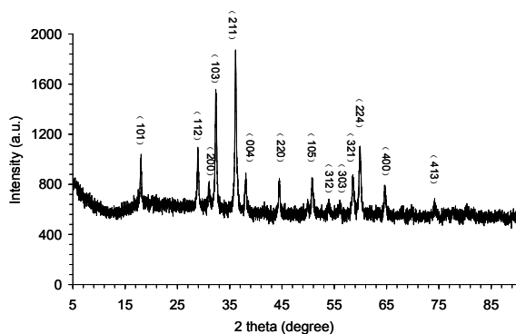
Figure S1. XRD pattern of \text{Mn}_3\text{O}_4 synthesized at 120^\circ\text{C} for 2h (sample S2).
