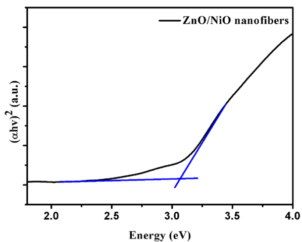
Fig.S1. the plots of the (\alpha h\nu)^2 vs photon energy ( h\nu ) for ZnO/NiO nanofibers.
