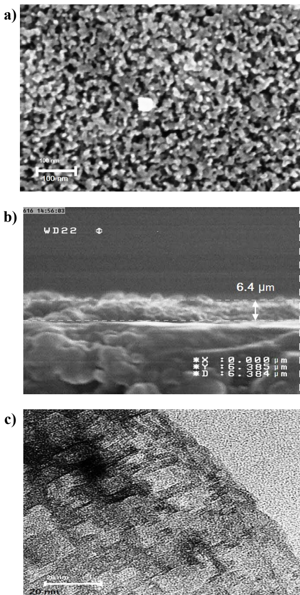
Figure S1: FE-SEM images from top (a) and cross section (b) of Hybrid-POM film. TEM image from Hybrid-POM nanoparticles.
