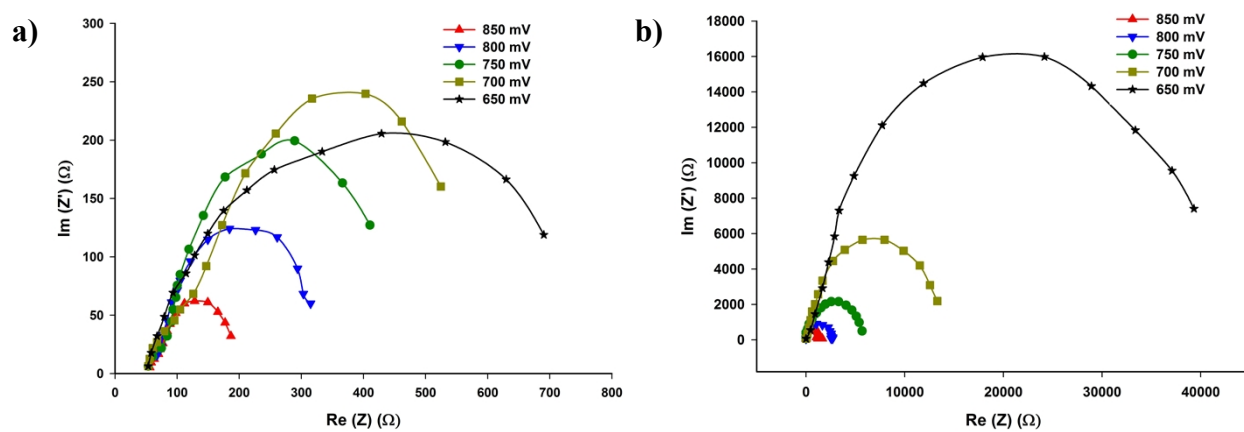
Figure S3: Nyquist EIS plots of DSCs with mp-TiO 2 (a) and Hybrid-POM (b), in the dark and different bias potentials.
