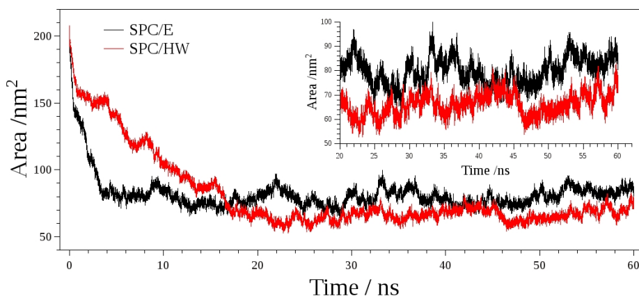
Fig.S2: Solvent Accessed Area (SAS) of a system of 70 SDS monomers in a l system of 70 SDS. The main figure and the insert shows Fig.S2
