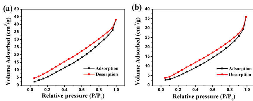
Fig. S3 Nitrogen adsorption and desorption isotherms of (a) NiCo 2 S 4 /RGO-3 hybrid and (b) NiCo 2 S 4 .
