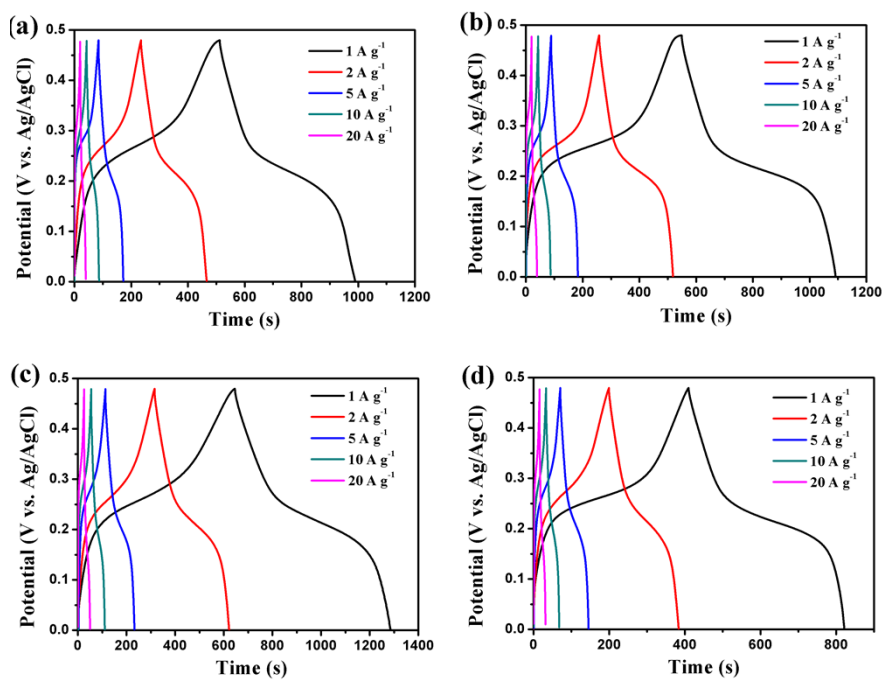
Fig. S4 Charge-discharge curves of (a) NiCo 2 S 4 /RGO-1, (b) NiCo 2 S 4 /RGO-2, (c) NiCo 2 S 4 /RGO-4, (d) NiCo 2 S 4 electrodes at various current densities of 1.0, 2.0, 5.0, 10 and 20 A g -1 .
