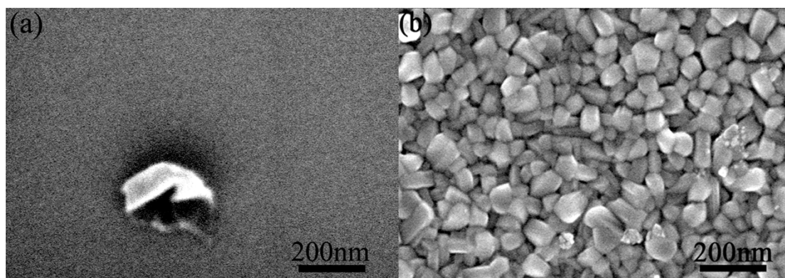
Fig. 2 (a) the top view of S4 before annealing, (b) the top view of S4 after annealing.
