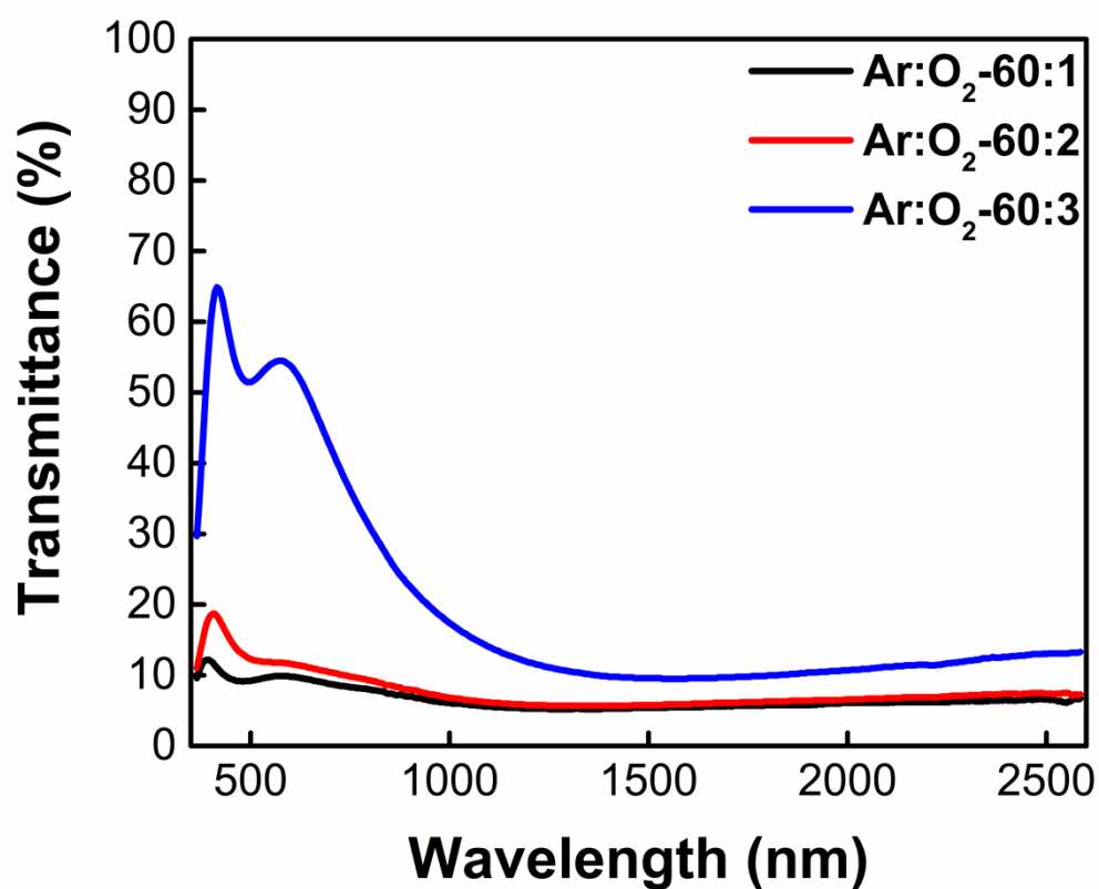
Fig.1 the transmittance spectrum of low oxygen ratio samples.
