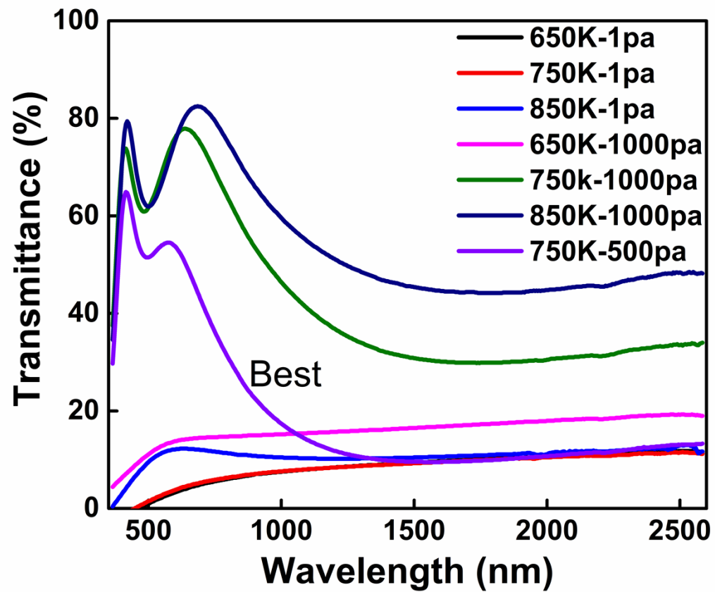
Fig.3 the transmittance spectrums with respect to pressure and temperature during annealing process.
