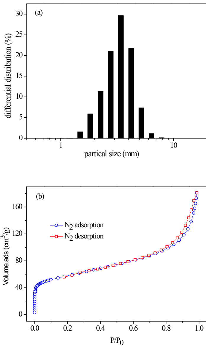
Fig. S1 Carbon black characteristics of (a) particle size and (b) N 2 adsorption/desorption isotherms
