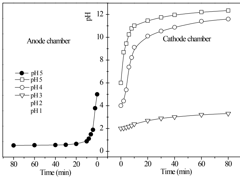
Fig. S2 Variation of pH value as the function of electrolytic time.
