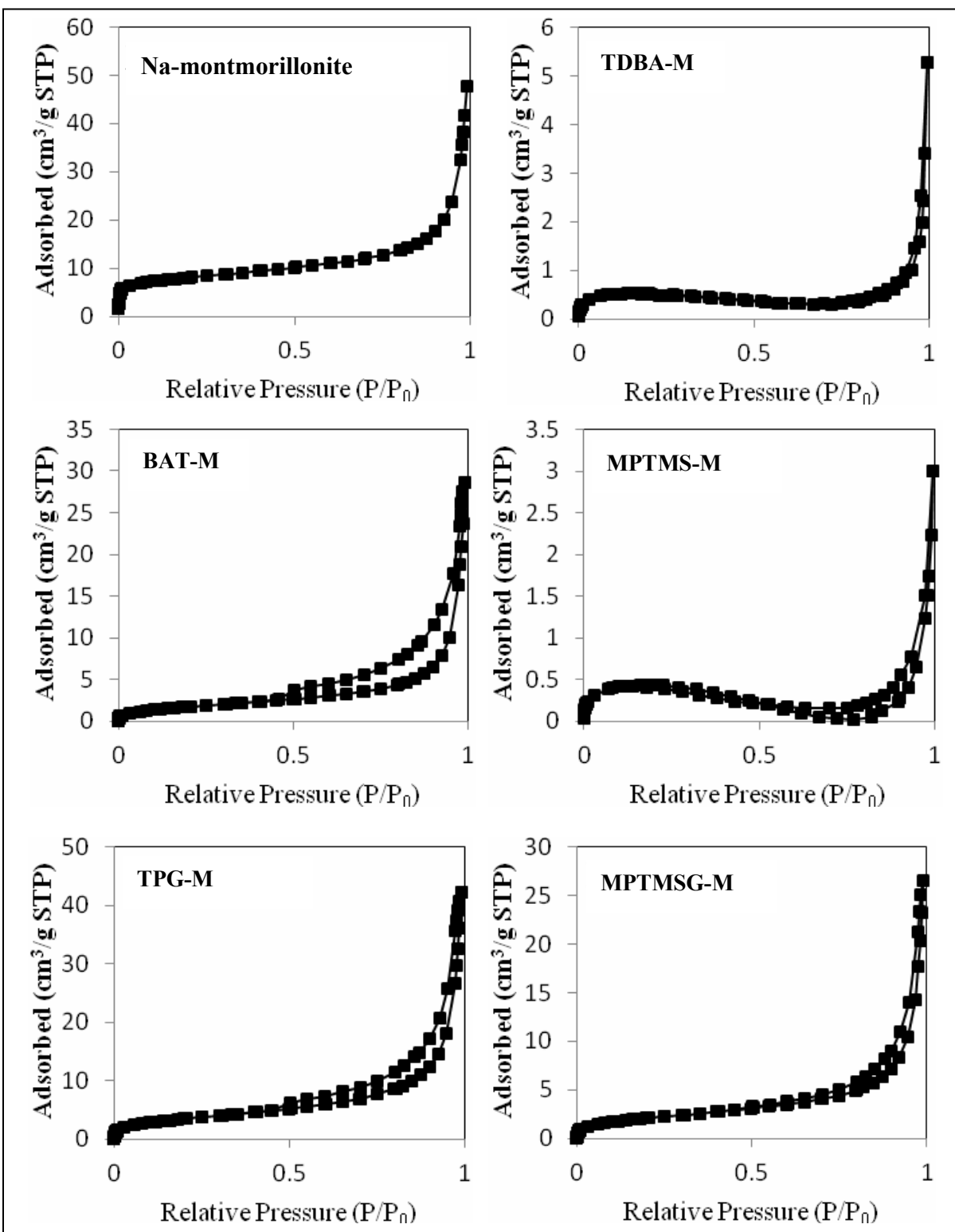
Fig. S1: N_2 adsorption isotherms of unmodified and modified montmorillonites
