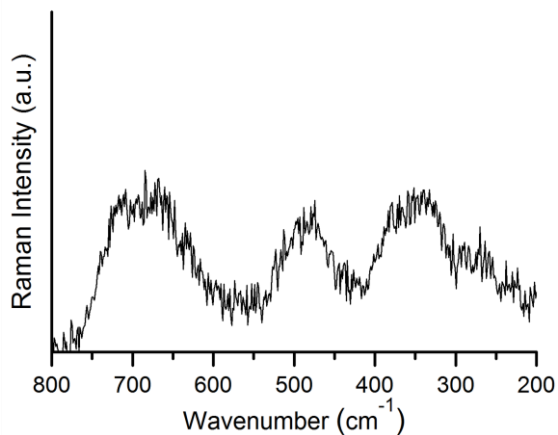
Figure S2. Raman spectrum of calcinated NWs
