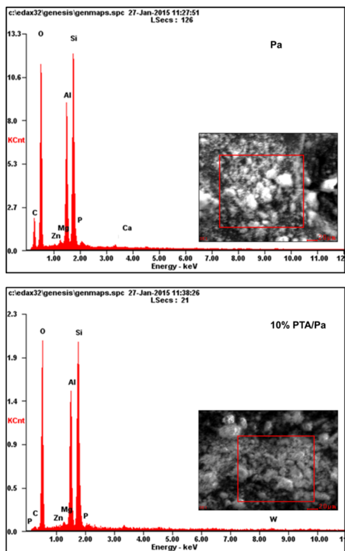
Fig. S1 EDX plots of Pa and PTA/Pa composite.
