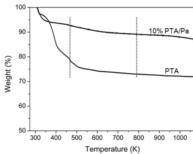
Fig. S3 TGA curves of PTA and 10% PTA/Pa composite.
