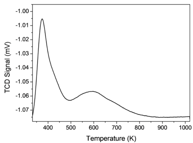
Fig. S2 \text{NH}_3 -TPD profile of H-Beta zeolite.
