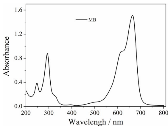
Fig. S3 The UV-vis of methylene blue
