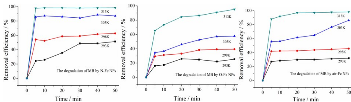
Fig. S3 The removal efficiency of MB using N-Fe NPs, O-Fe NPs and air-Fe NPs, respectively.
