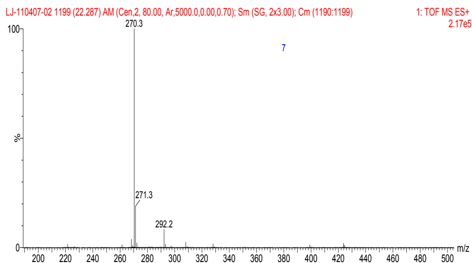
Fig. B-24 MS-ESI spectrum of picolinaldehyde oximyl 4-isopropylcyclohexa -1, 3-dienecarboxylate
