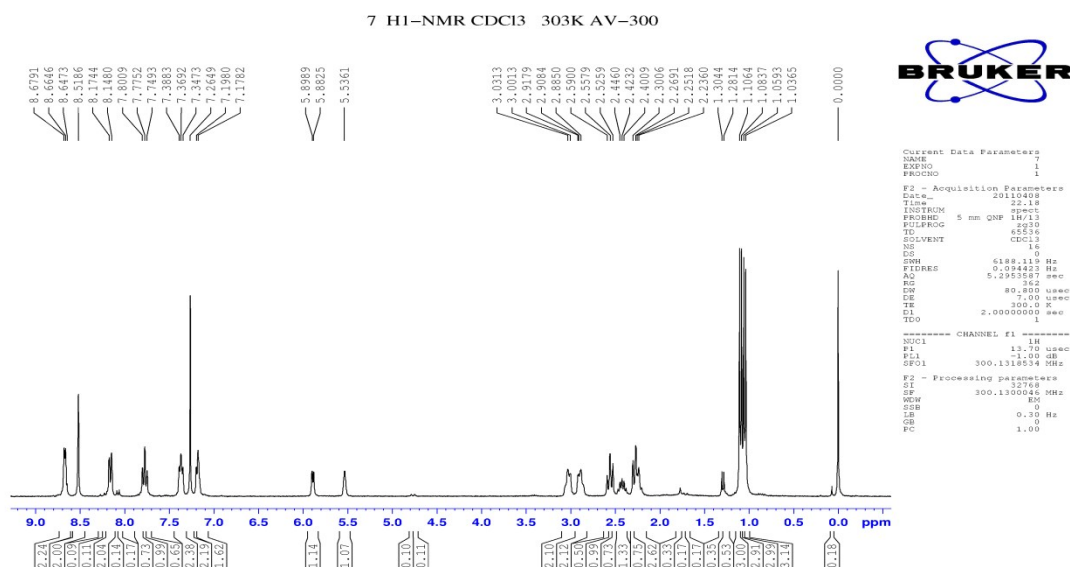
Fig. B-16 1 H NMR spectrum of picolinaldehyde oximyl 4-isopropylcyclohexa-1, 3-dienecarboxylate
