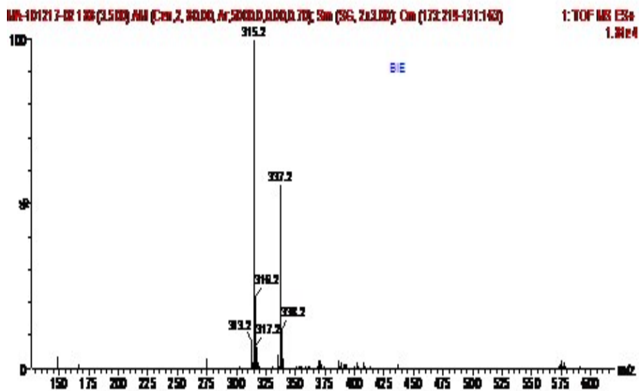
Fig.B-20 MS-ESI spectrum of N-benzyl-2-(4-isopropylcyclohexa-1, 3-dienyl)-2-oxoethanethioamide
