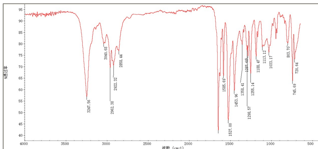
Fig. B-2 FTIR spectrum of 4-isopropyl-N-(o-methylphenyl) cyclohexa-1, 3-dienecarboxamide
