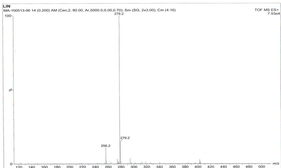
Fig. B-18 MS-ESI spectrum of 4-isopropyl-N-(o-methylphenyl)cyclohexa-1, 3-dienecarboxamide
