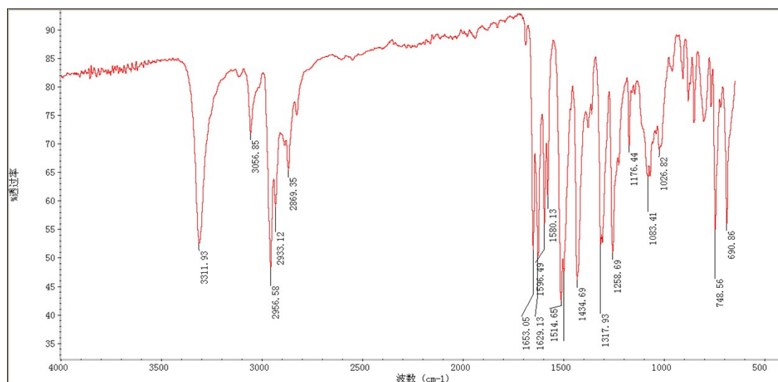
Fig. B-1 FTIR spectrum of 4-isopropyl-N-phenylcyclohexa-1, 3-dienecarboxamide
