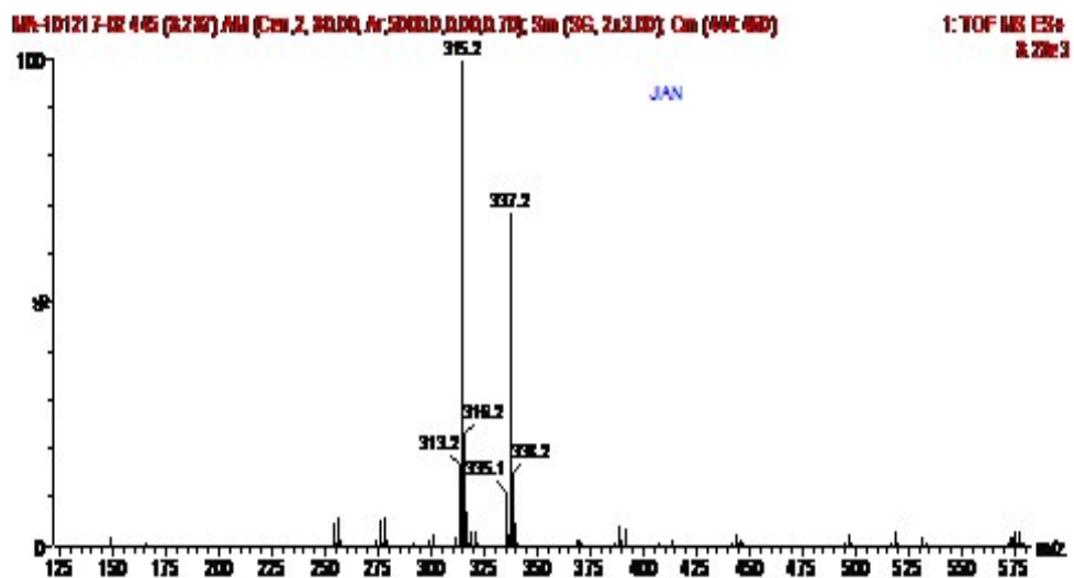
Fig. B-21 MS-ESI spectrum of 2-(4-isopropylcyclohexa-1,3-dienyl) -2-oxo-N-m-tolylethanethioamide
