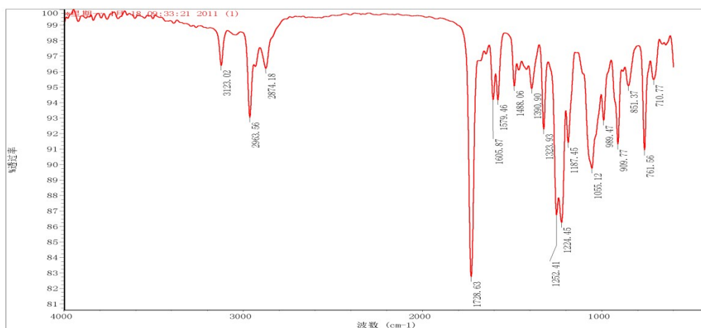
Fig. B-6 FTIR spectrum of 1-(unan-2-yl) ethanone oximyl 4-isopropylcyclohexa-1, 3-dienecarboxylate
