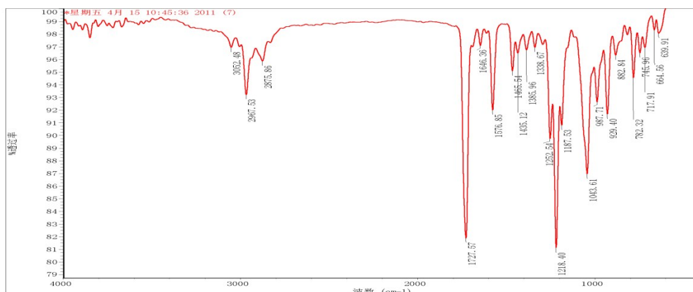
Fig. B-8 FTIR spectrum of picolinaldehyde oximyl 4-isopropylcyclohexa-1, 3-dienecarboxylate 3-dienecarboxamide
