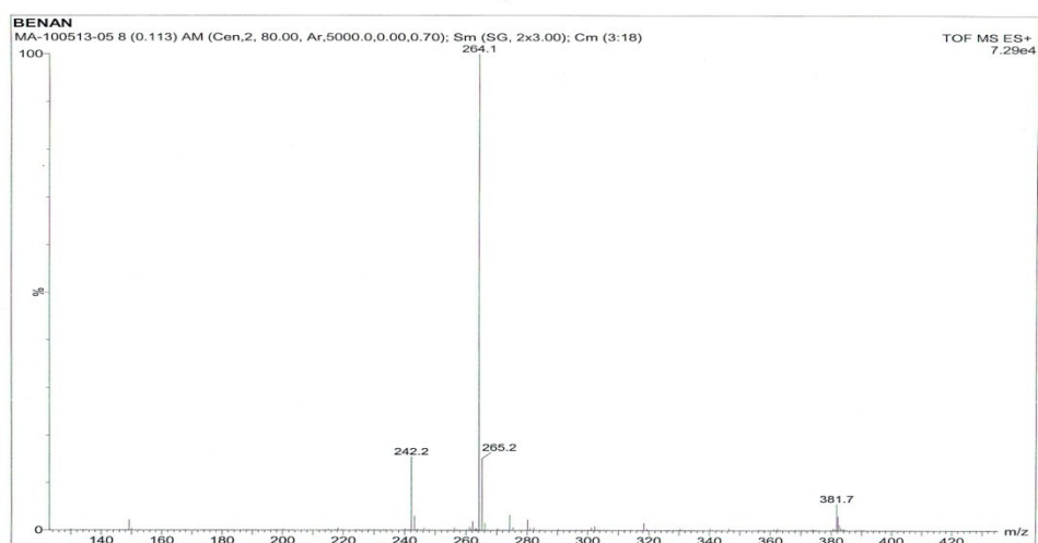
Fig. B-17 MS-ESI spectrum of 4-isopropyl-N-phenylcyclohexa-1, 3-dienecarboxamide
