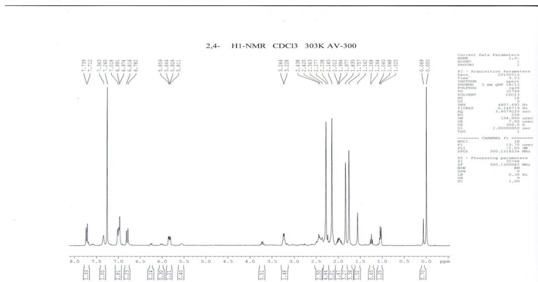
Fig. B-11 1 H NMR spectrum of 4-isopropyl-N-(2, 4-methylphenyl) cyclohexa-1, 3-dienecarboxamide
