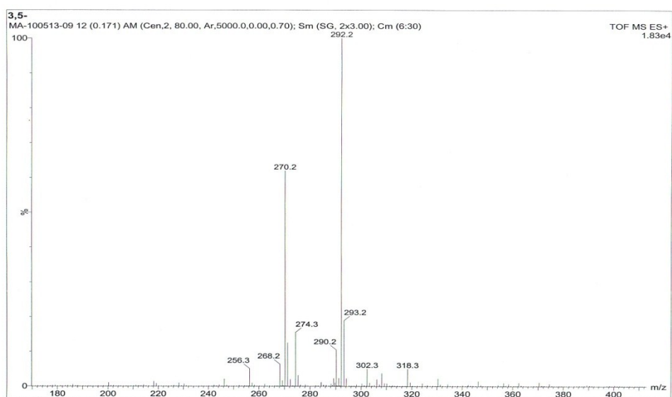
Fig. B-19 MS-ESI spectrum of 4-isopropyl-N-(2, 4-methylphenyl) cyclohexa-1, 3-dienecarboxamide
