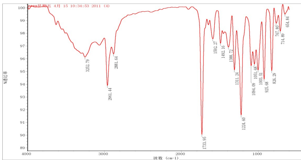
Fig. B-7 FTIR spectrum of 1-(4-chlorophenyl) ethanone oximyl 4-isopropylcyclohexa-1, 3-dienecarboxylate
