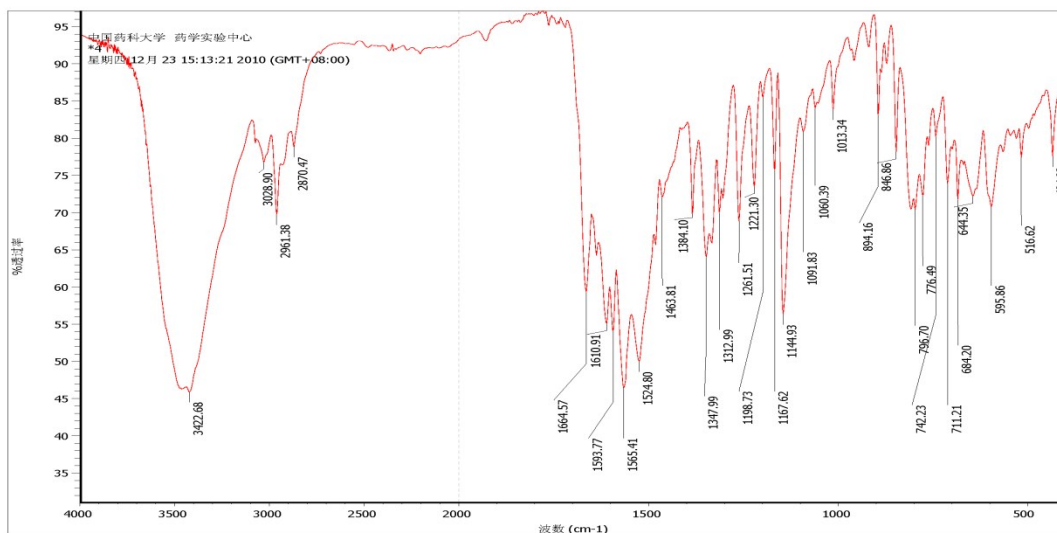
Fig. B-5 FTIR spectrum of 2-(4-isopropylcyclohexa-1,3-dienyl)-2-oxo-N-m-tolyethanethioamide
