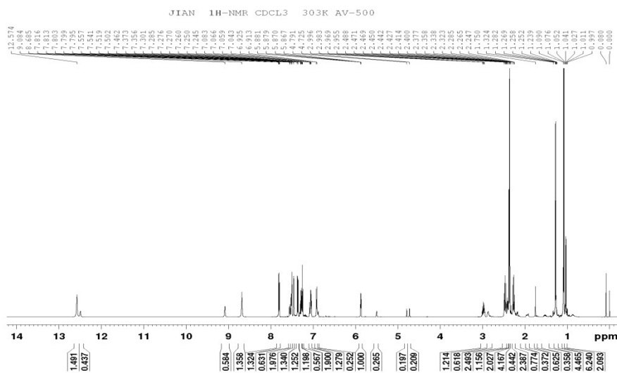
Fig. B-13 1 H NMR spectrum of 2-(4-isopropylcyclohexa-1, 3-dienyl) -2-oxo-N-m-tolylethanethioamide
