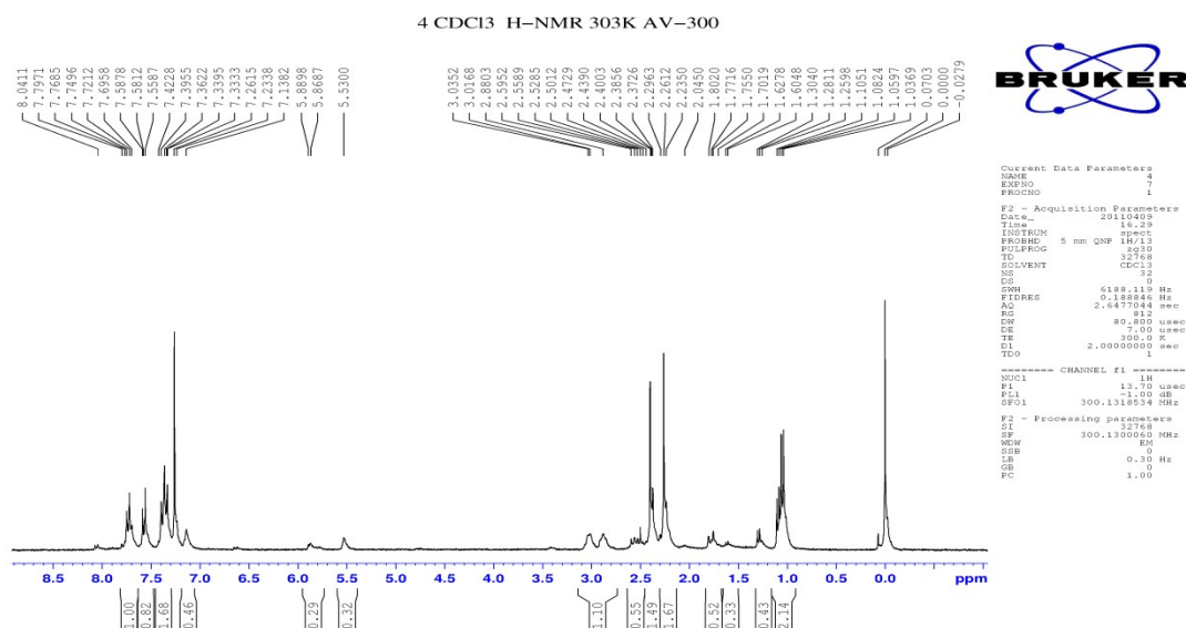
Fig. B-15 1 H NMR spectrum of 1-(4-chlorophenyl) ethanone oximyl 4-isopropylcyclohexa-1, 3-dienecarboxylate
