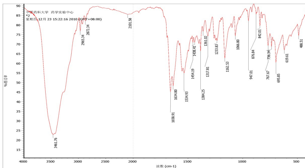
Fig. B-4 FTIR spectrum of N-benzyl-2-(4-isopropylcyclohexa-1,3-dienyl)-2-oxoethanethioamide
