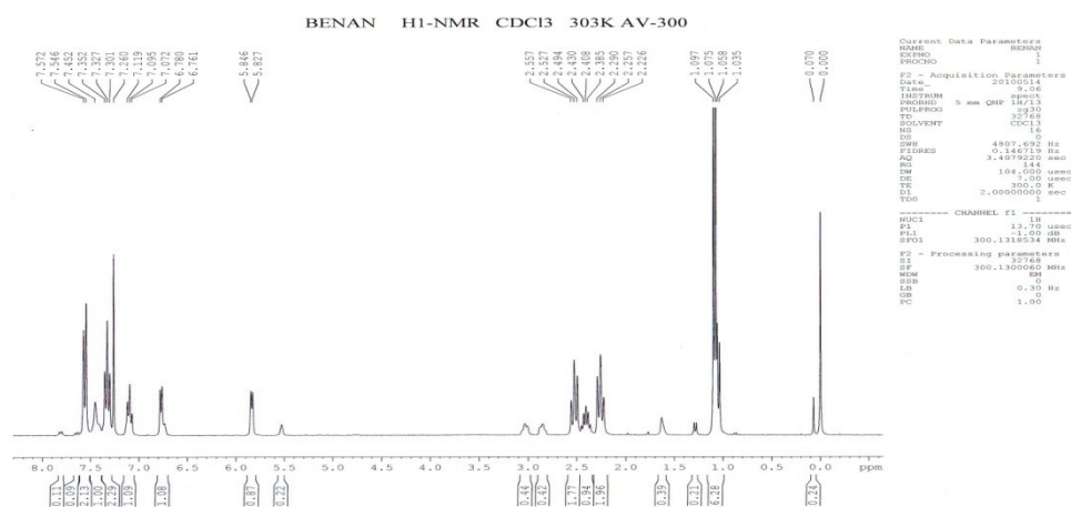
Fig. B-9 ^1\text{H} NMR spectrum of 4-isopropyl-N-phenylcyclohexa-1, 3-dienecarboxamide
