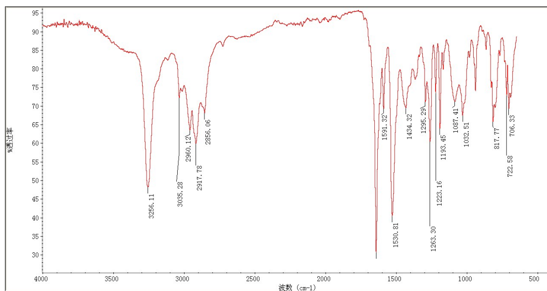
Fig. B-3 FTIR spectrum of 4-isopropyl-N-(2, 4-methylphenyl) cyclohexa-1, 3-dienecarboxamide
