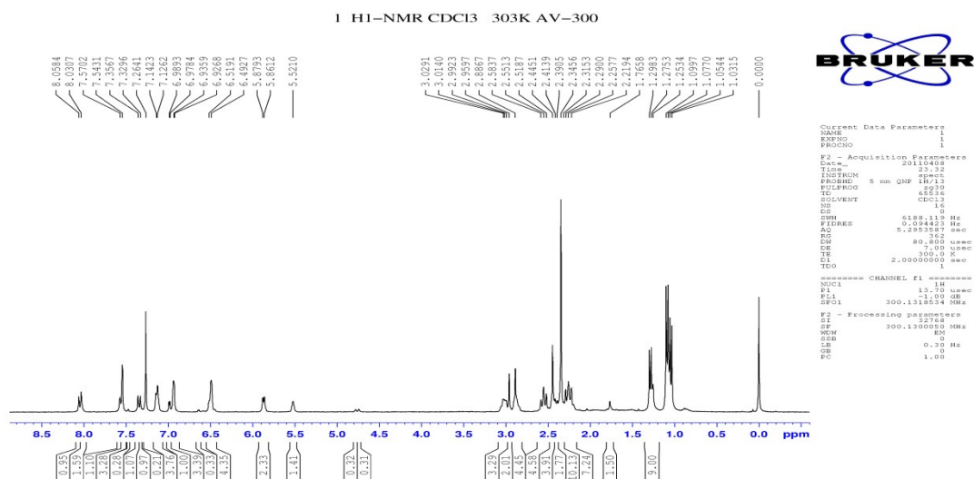
Fig. B-14 1 H NMR spectrum of 1-(funan-2-yl) ethanone oximyl 4-isopropylcyclohexa-1,3-dienecarboxylate
