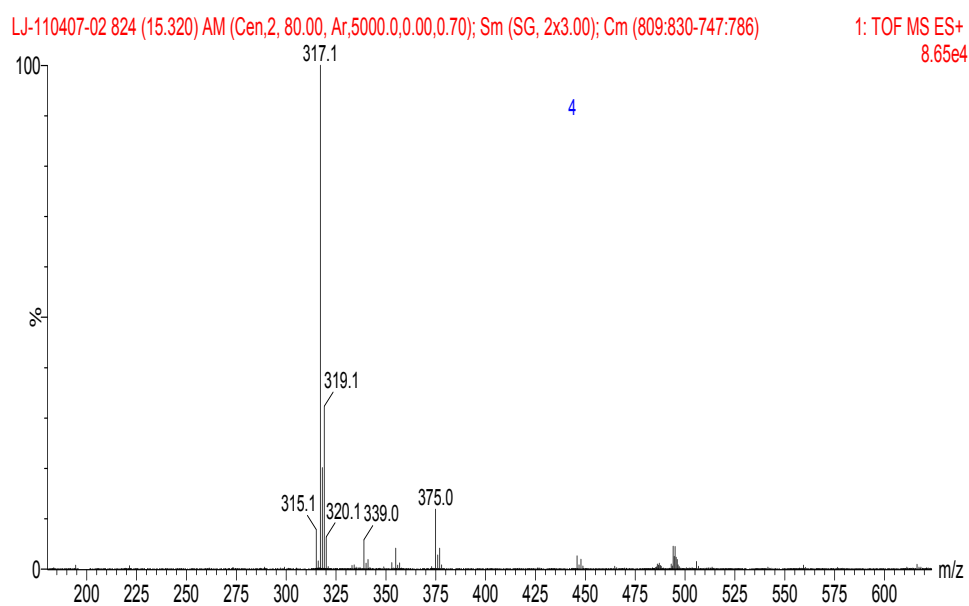
Fig. B-23 MS-ESI spectrum of 1-( 4-chlorophenyl) ethanone oximyl 4-isopropylcyclohexa-1, 3 -dienecarboxylate
