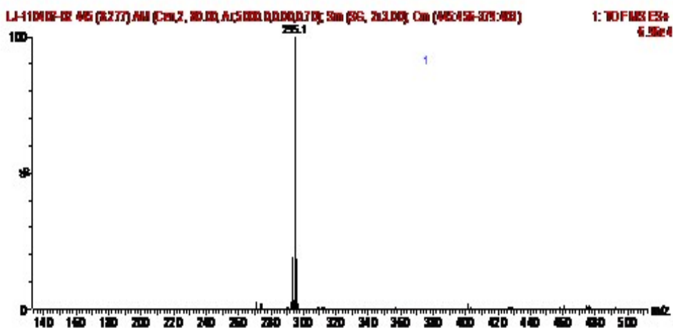
Fig. B-21 MS-ESI spectrum of 2-(4-isopropylcyclohexa-1,3-dienyl) -2-oxo-N-m-tolylethanethioamide
