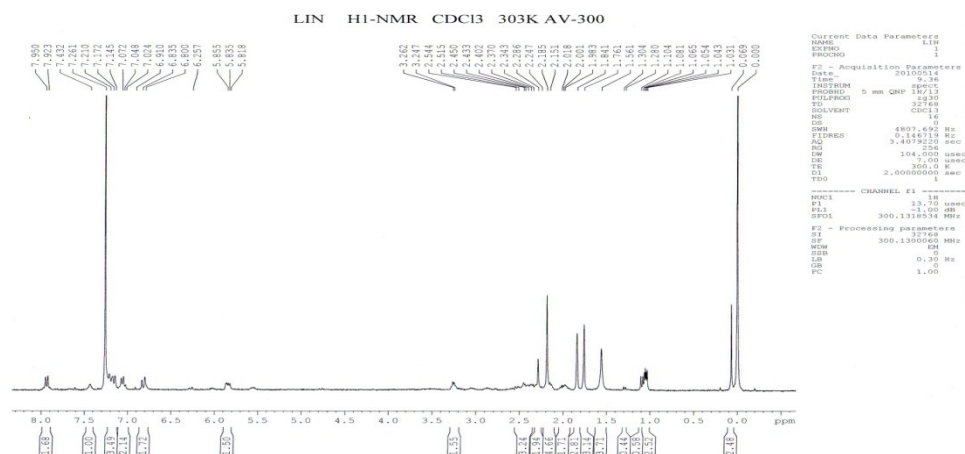
Fig. B-10 ^1\text{H} NMR spectrum of 4-isopropyl-N-(o-methylphenyl) cyclohexa-1, 3-dienecarboxamide
