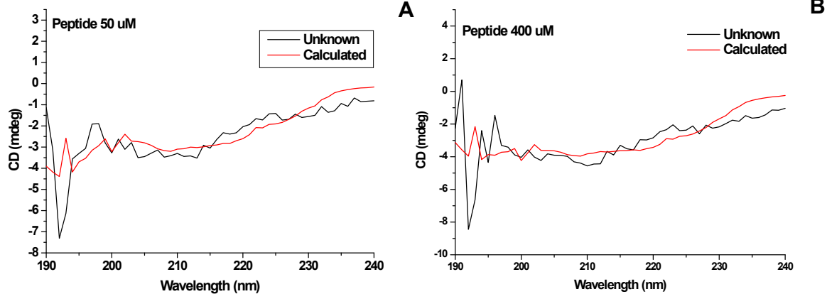
Supplementary Figure 2: CD spectra showing secondary structures of KLVFF peptide at different concentrations [A] 50 \mu\text{M} and [B] 400 \mu\text{M}
