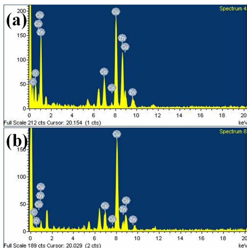
Figure S1. EDS spectrum of (a) 5 and b) 10 at. % Co: ZnO NPs.
