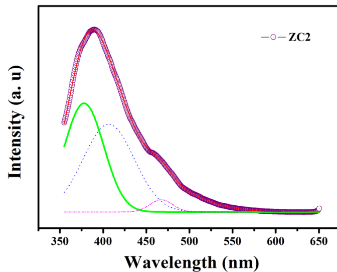
Figure S2. Gaussian deconvoluted emission spectrum of 5 at. % Co: ZnO NPs. Hollow circles-experimental data, red solid line-Gaussian fitting, Green, blue and pink lines-band edge, neutral and ionized Zn vacancy emissions.
