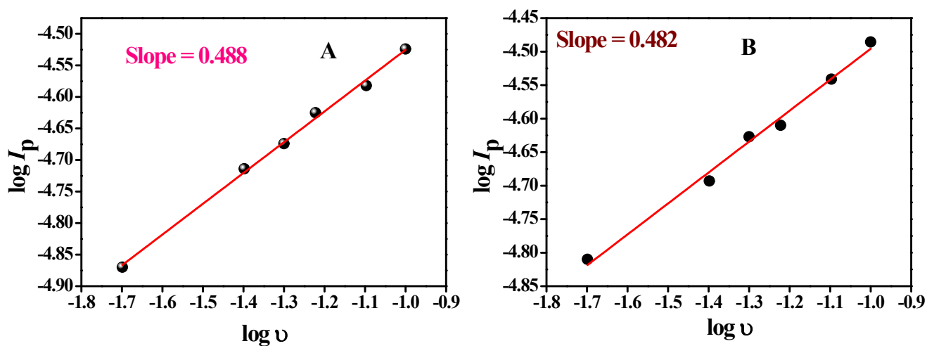
Fig. S2. \log of I_p versus \log of scan rate plots for (A) 4-APA and (B) 4-ABA at 308K
