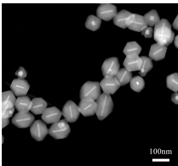
Figure S1 STEM image of OCT-Au@Cu 2 O
