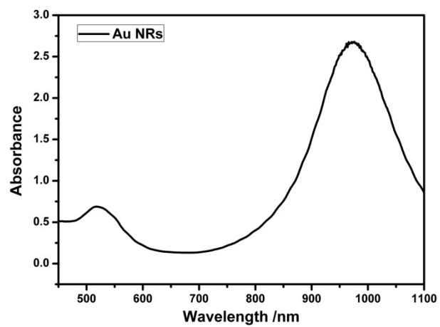
Figure S2 UV-vis absorption spectrum of Au NRs
