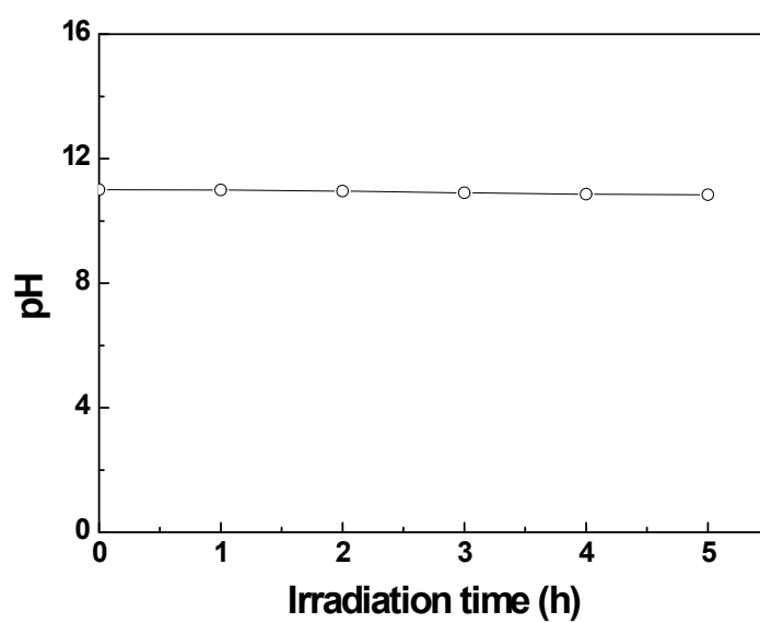
Fig. S3. Time-dependent pH of EDTA-Ni solution during hydrogen evolution (SiNWs: 3 cm × 3 cm; length of nanowires: 4 \mu\text{m} ; EDTA-Ni aqueous solution: 0.025 mol·L -1 100 mL; initial pH: 11; irradiation time: 5 h).
