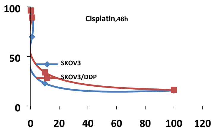
Fig. S1. Representative dose-dependent cell viability curve of cisplatin on cisplatin-sensitive Human ovarian cancer SKOV3 cells and cisplatin-resistant human ovarian cancer SKOV3/DDP cells (mean \pm SD, n=3).
