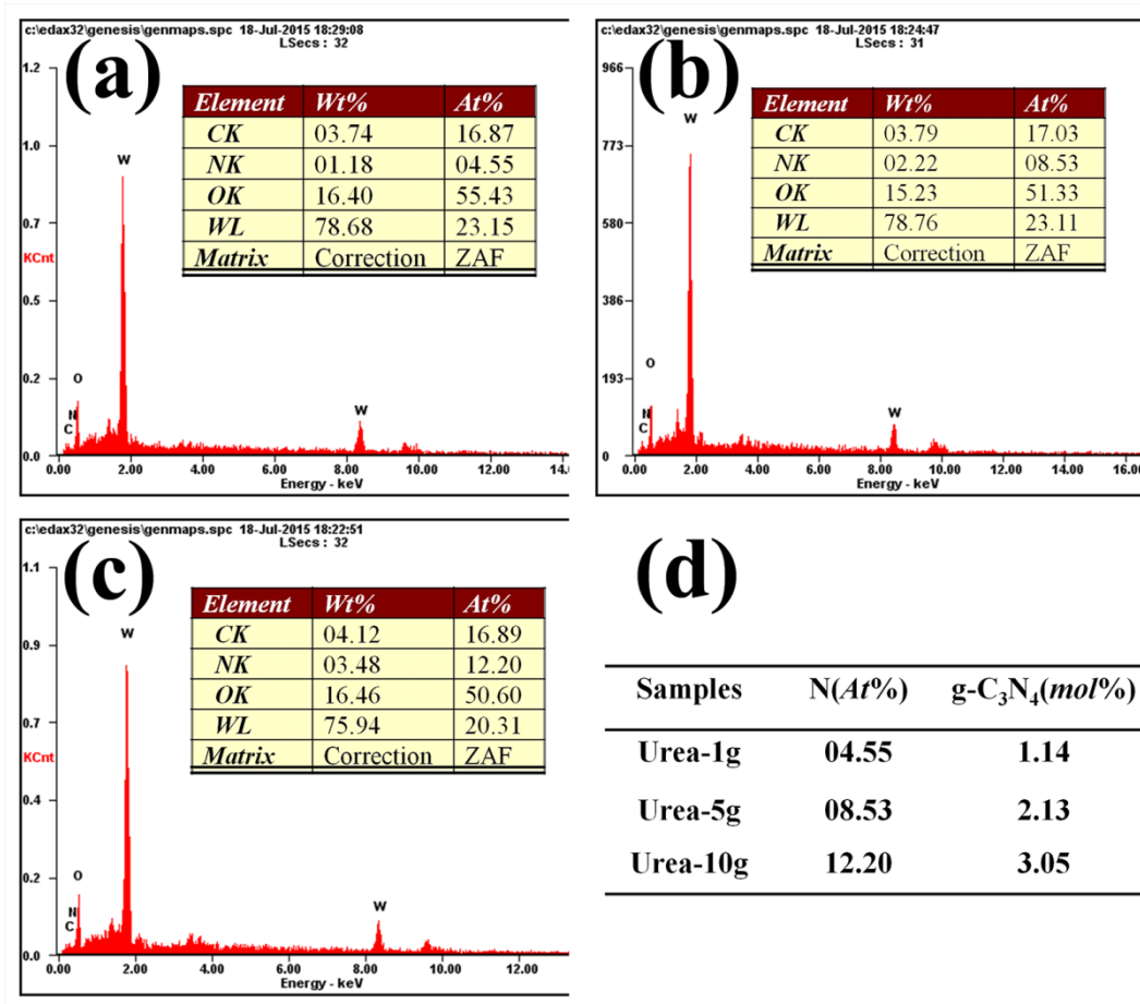
Fig.S1 The EDS analysis of g-C 3 N 4 /WO 3 films prepared with different weight of urea-1g (a), 5g (b), and 10g (c), and the corresponding g-C 3 N 4 content (d).
