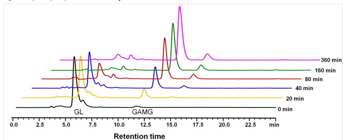
Fig. S4 Hydrolysis process of GL by PGUS.
