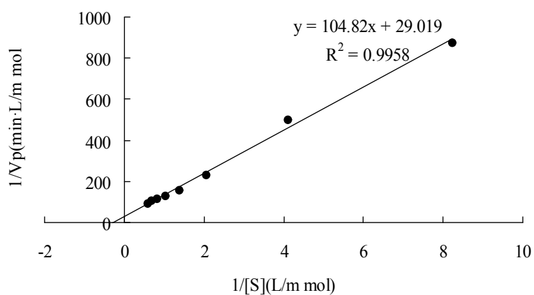
Fig. S3 Lineweaver- Burk plot of GL hydrolysis by AuGUS .
