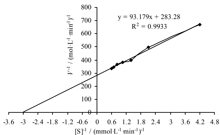
Fig. S1 Lineweaver- Burk plot of GL hydrolysis by PGUS .
