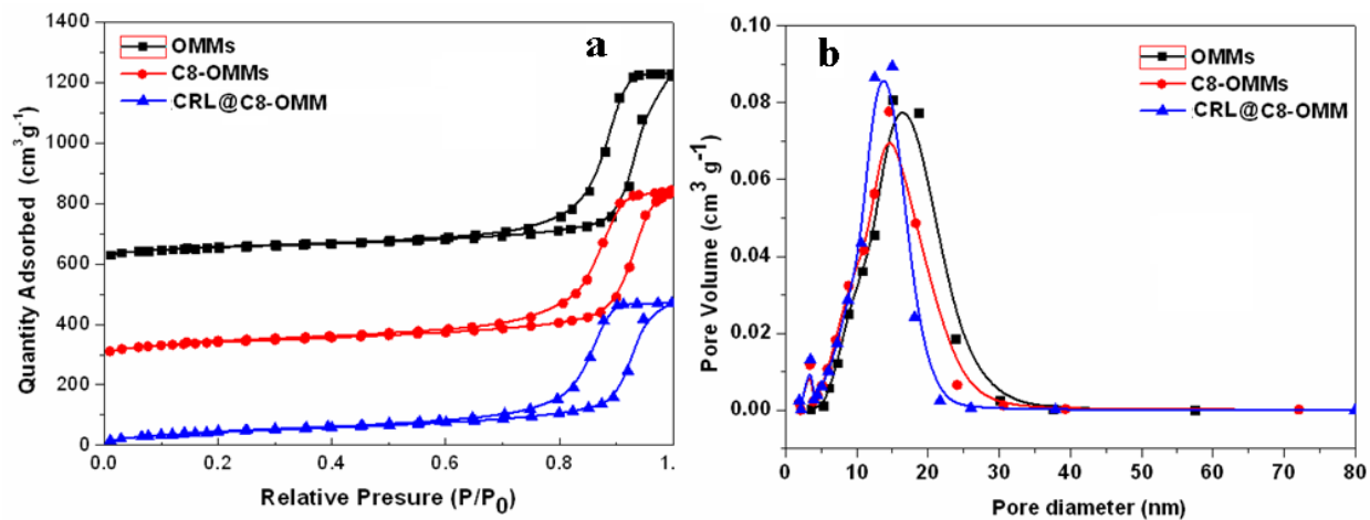
Fig. S1. Isotherms (a) and pore diameter distributions (b) of the OMMs, C8-OMMs and CRL@C8-OMMs.
