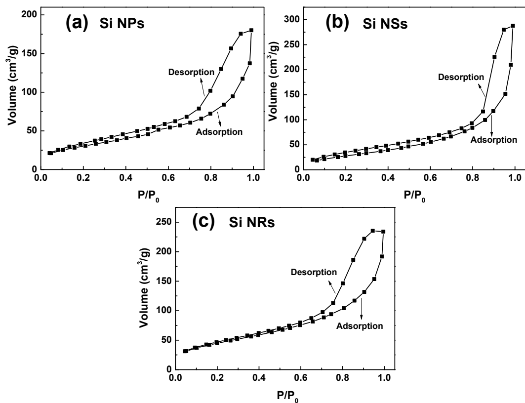
Fig. S1. Nitrogen adsorption-desorption isotherms of (a) Si NPs, (b) Si NSs, (c) Si NRs under 77.3 K.
