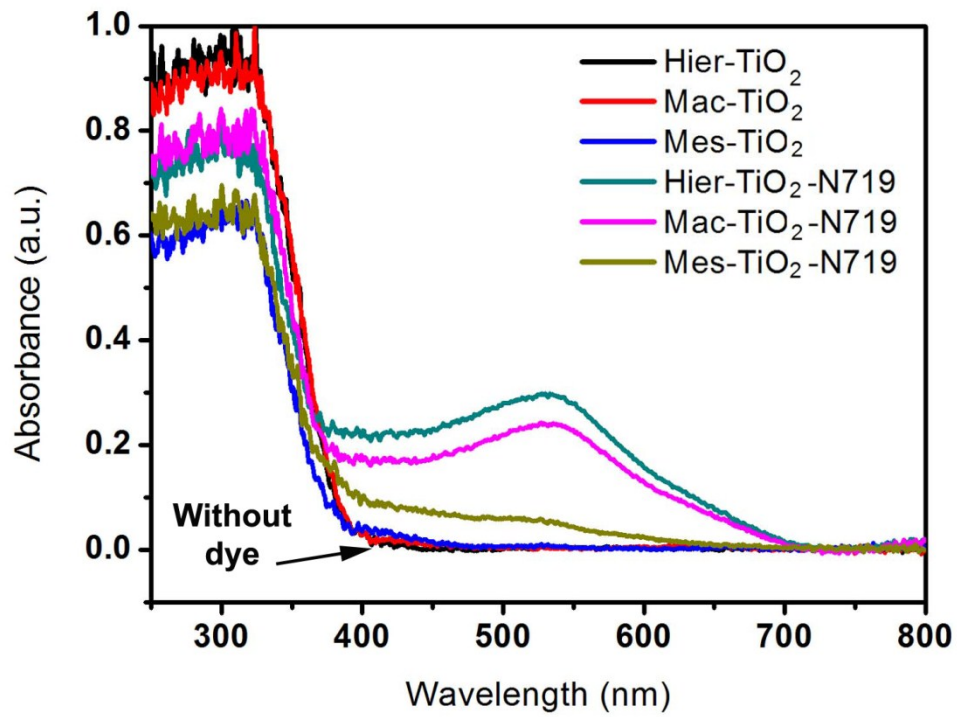
Figure S2. UV-DRS spectra of the photoanodes with and without dye loading.
