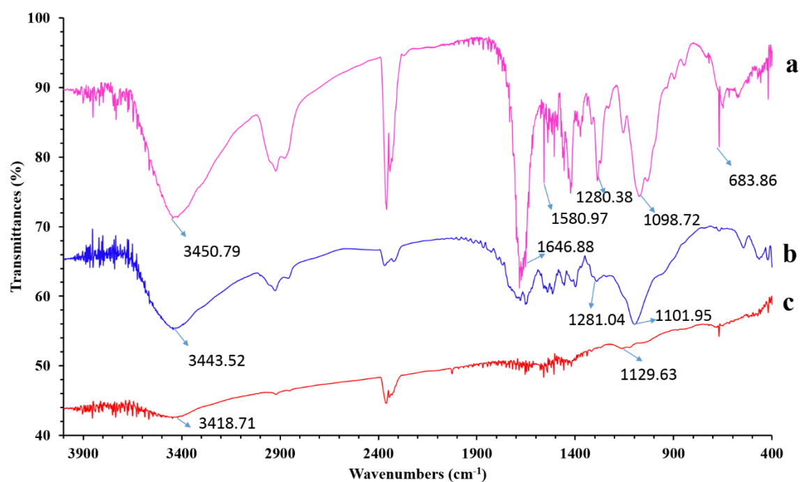
Supplementary information Fig. 1 FTIR spectra of CP/CNT/DA-MIM (a), CP-MIM (b) and activated MWCNT (c).
