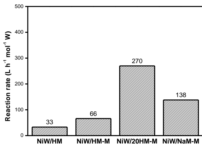
Figure SI-1 : Catalytic performance for thiophene HDS of various hierarchical Mordenite supported NiW catalysts (Acronym have the same signification than for NiW/HB catalysts).
