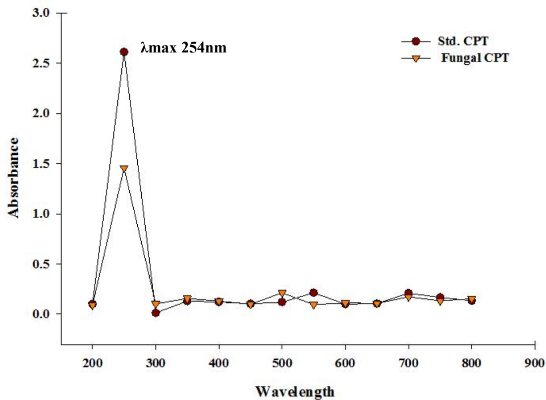
Fig. 1: UV-Spectrum of authentic/standard CPT and extracted CPT produced by endophytic fungus.
