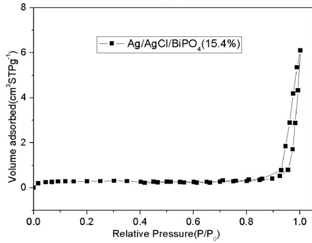
Fig. S1. N 2 adsorption–desorption isotherms of BiPO 4 and Ag/AgCl/BiPO 4 (15.4%).
