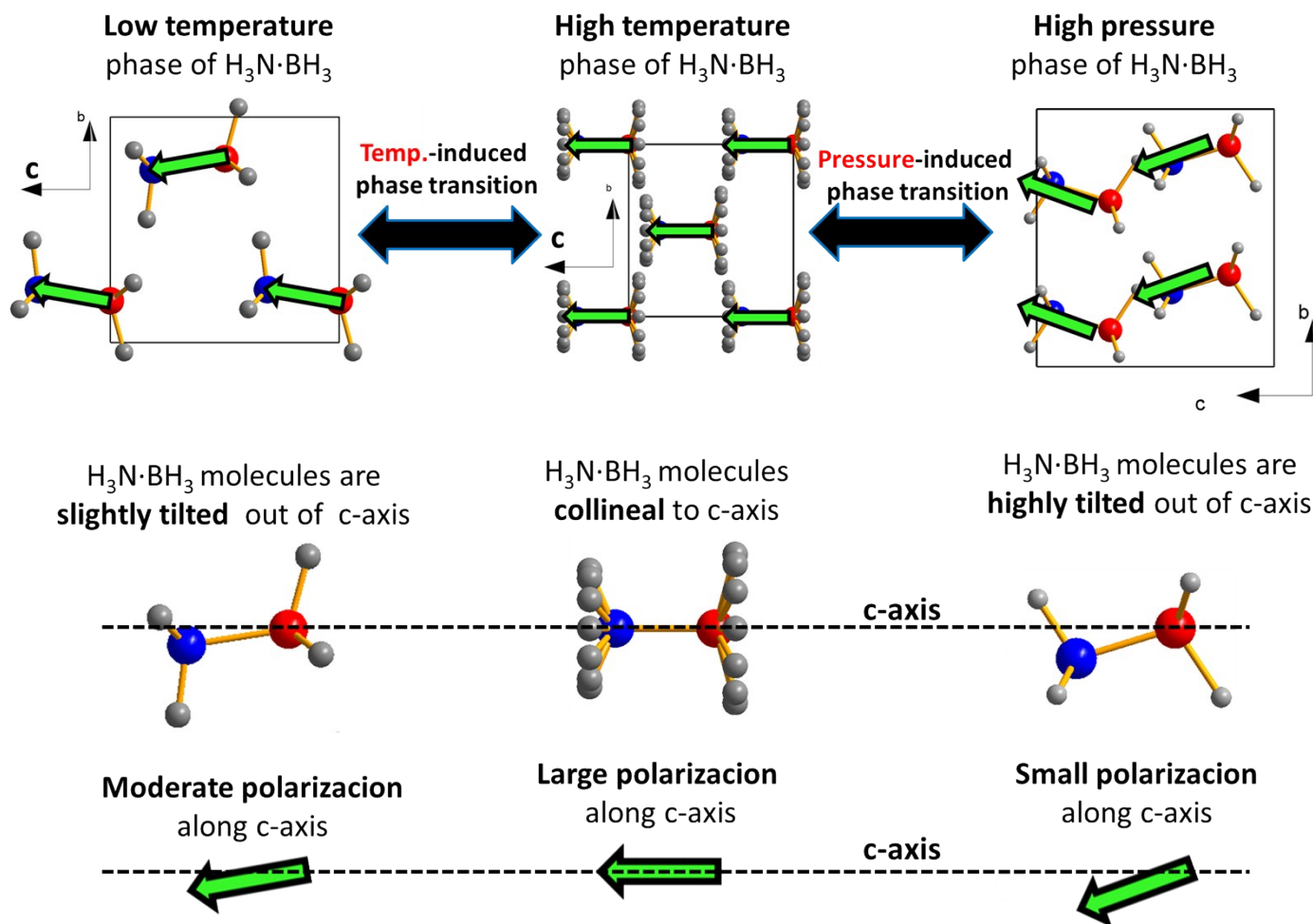
Figure S2. Scheme of phase transitions induced by temperature and pressure on ammonia-borane crystals. Also, we show the arrangement of ammonia-borane molecules and associated dipole moments along the c-axis.
