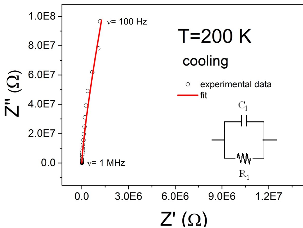
Figura S1.- Typical impedance complex plane of ferrocene and its corresponding fit representative of the temperatures around the transition and below.
