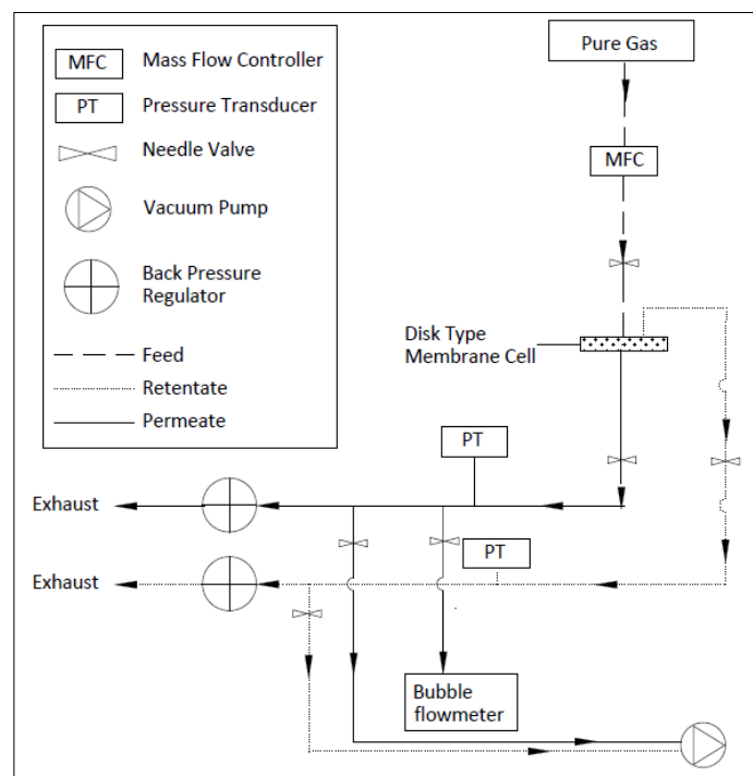
Fig. S1 Schematic of the gas permeation setup.
