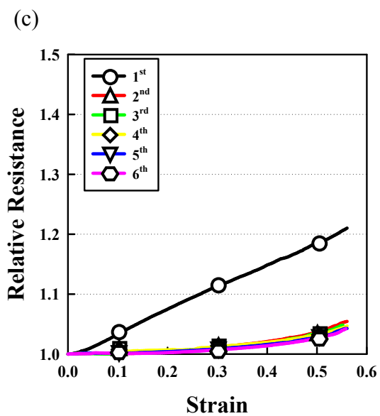
Figure S2. Repeatability test for 1 h-sonicated CNT-interlayered PDMS.
