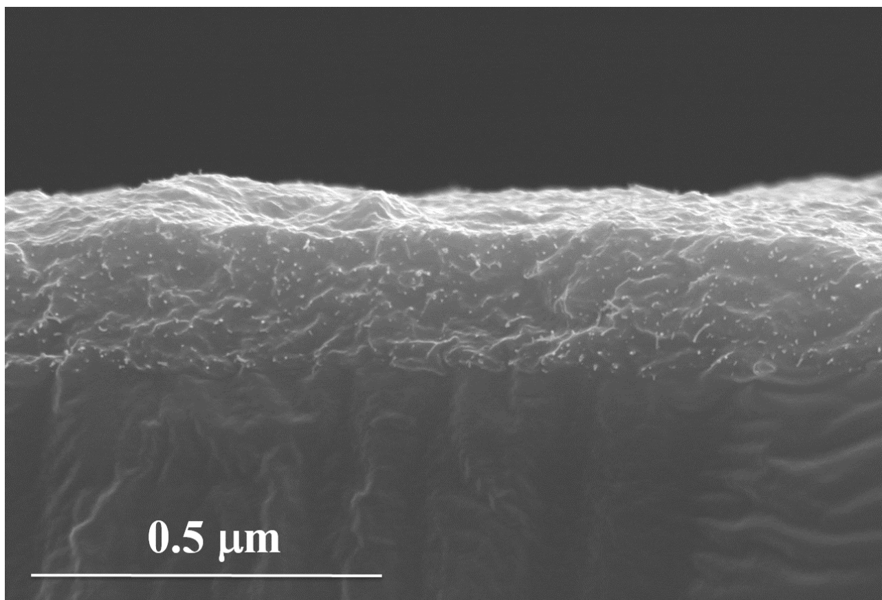
Figure S3. SEM images of higher magnification at the point of contact of the CNT film with the PDMS sheet
