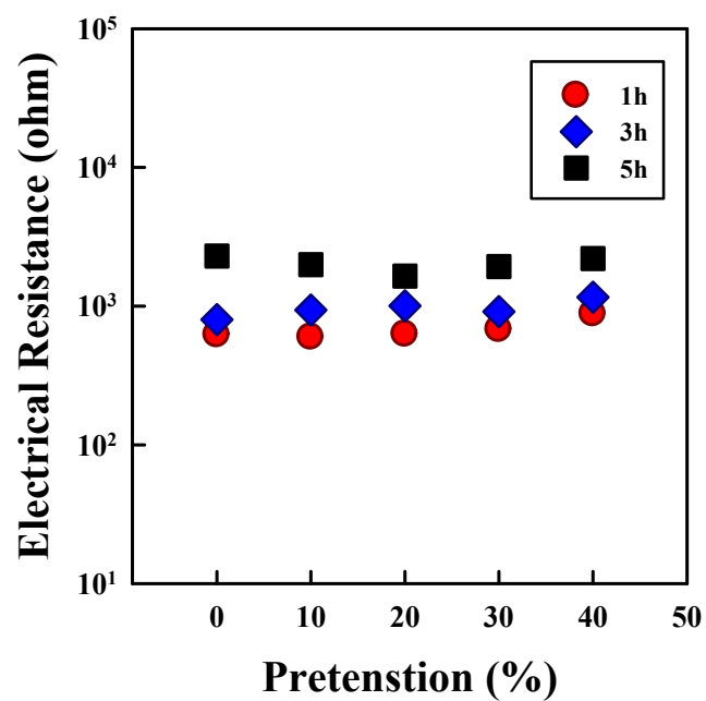
Figure S1. Electrical resistance of samples without elongation for various sonication times.
