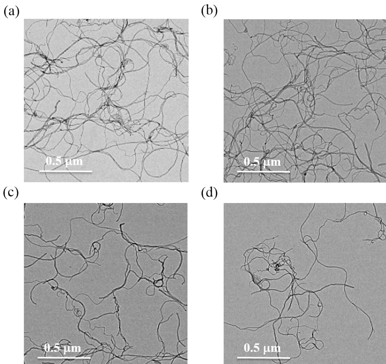
Figure S4. TEM images of CNTs after sonication for (a) 0h, (b) 1h, (c) 3h, and (d) 5h
