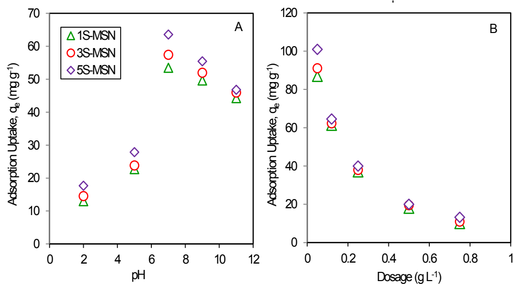
Fig. S1 (A) Effect of pH and (B) S-MSN dosage on adsorption of MB
