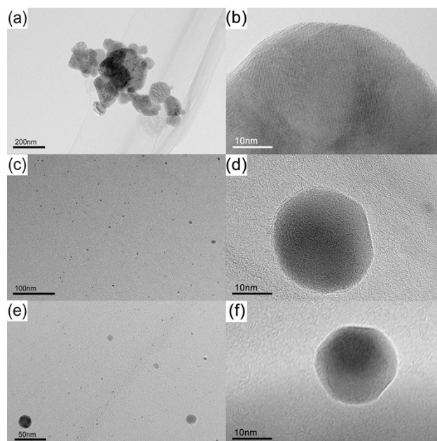
Fig. S1. HRTEM images of respective sample: (a-b) MBC800, (c-d) MBC1000 and (e-f) MBC1200.
