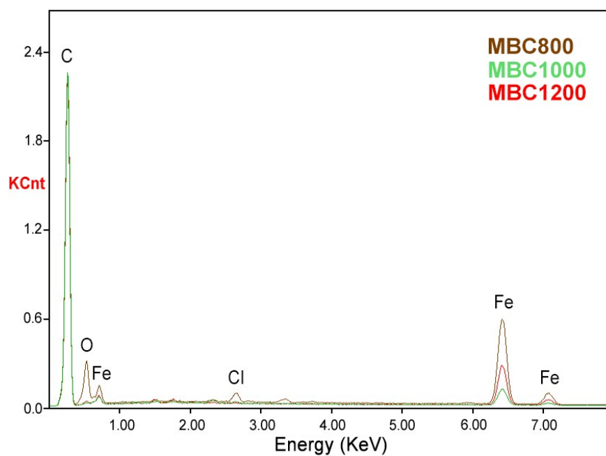
Fig. S2. EDAX spectra of MBC800, MBC1000 and MBC1200.
