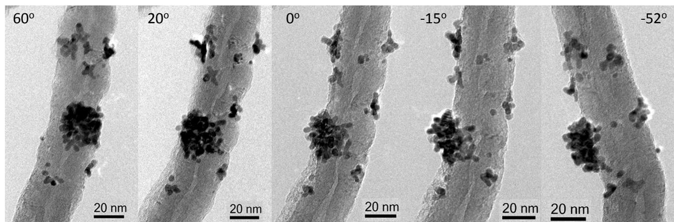
Figure S2. Selected bright field images of TEM tilt series obtained by tilting the TNCNT/ Pt sample to different angles: +60°, +20°, 0°, -15° and -52°.
