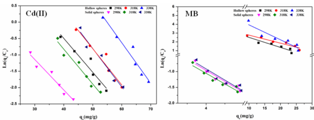
Fig. S1 Plots of \ln(q_e/C_e) as a function of q_e for Hollow spheres and Solid spheres at various temperature
