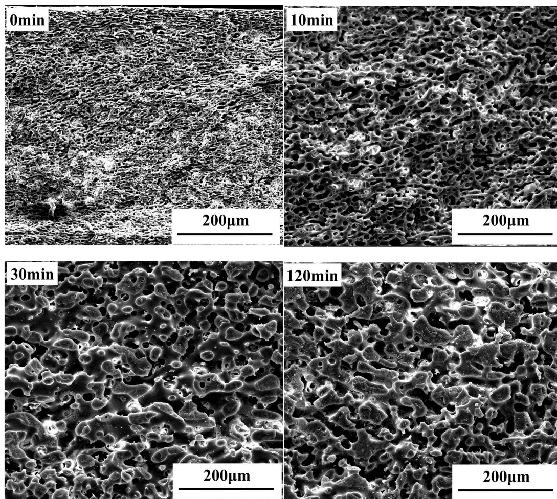
Fig. S1 SEM micrographs of 4wt% R974 nano- SiO 2 particle filled 50/50 PP/PS blend after annealing at 190 °C for various time.
