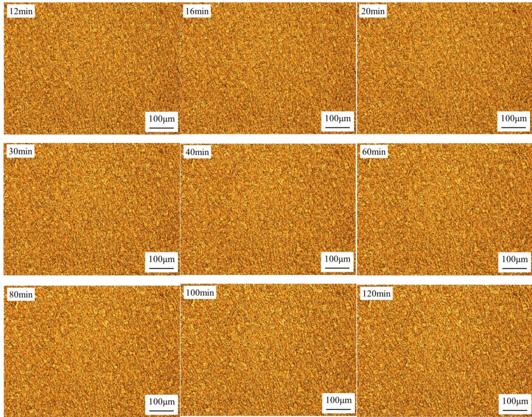
Fig. S2 Morphology evolution of 4wt% nano- SiO 2 particle filled 50/50 PP/PS blend observed by an optical microscope during annealing at 190 °C.
